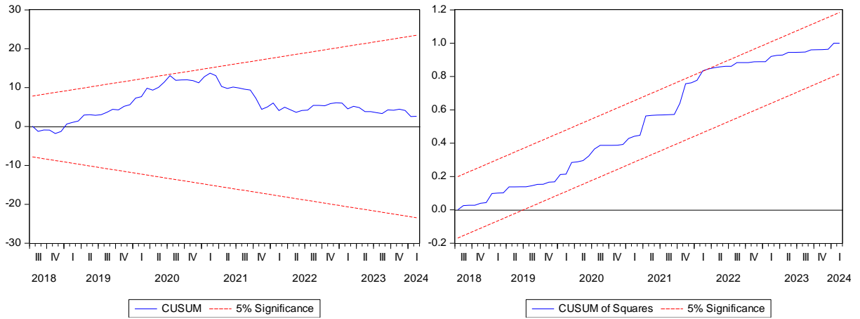
Figure 2. Stability Test for ROA
