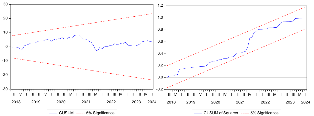
Figure 3. Stability Test for NOM
