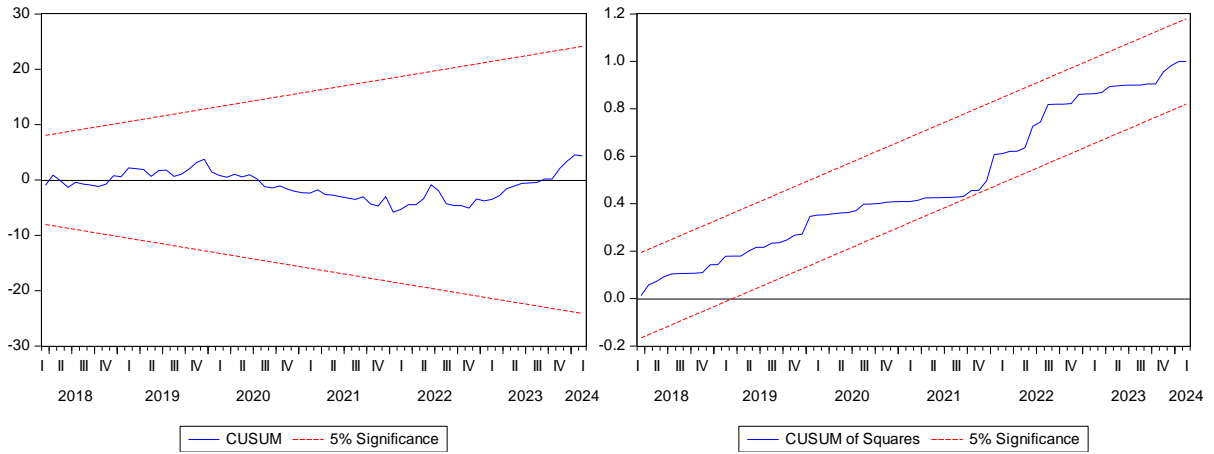
Figure 1. Stability Test for IPR
